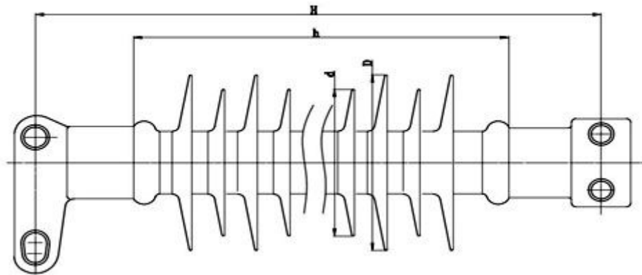
Fig. 110KV 5KN Composite Suspension Insulator
