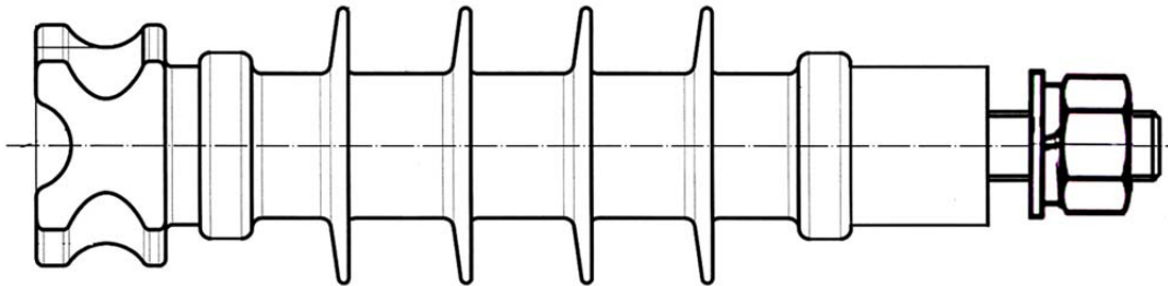
Fig. 11KV 10KN Composite Line Post Insulator
