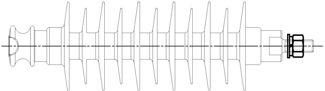
Fig. 33KV 10KN Composite Pin Insulator
