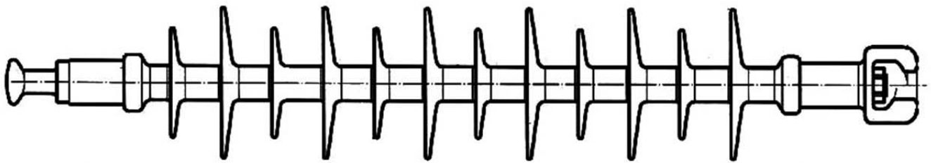
Fig. 33KV 70KN Composite Suspension Insulator
